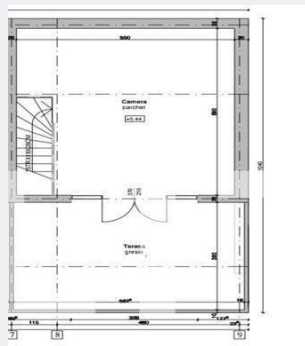
PLAN MANSARDA
