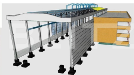
Macheta 3 D structura hala C3
