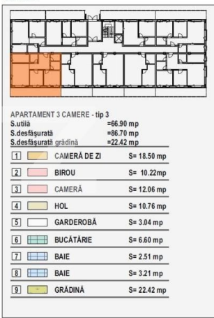
PLAN PARTER
